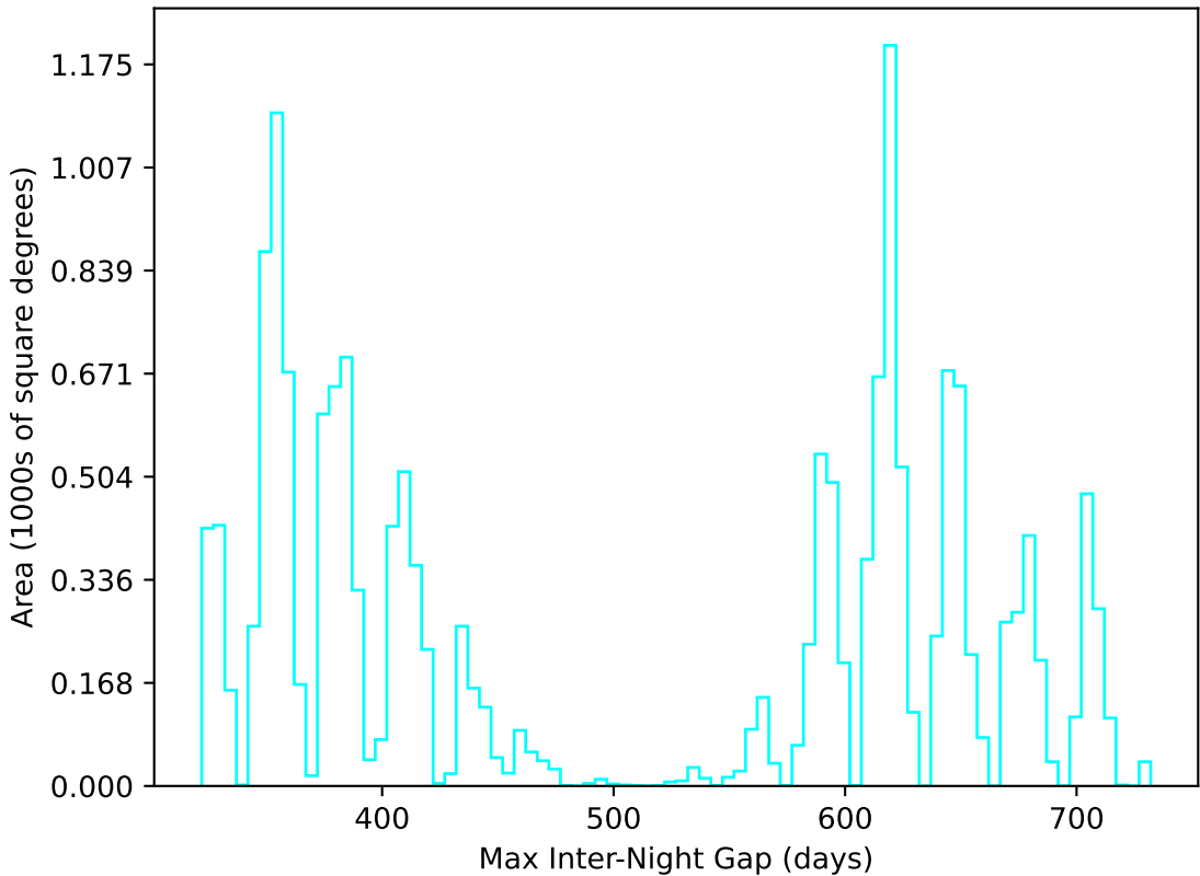
too_elab_r64_d2_giz_v3.4_10yrs WFD u band: Max Inter-Night Gap
