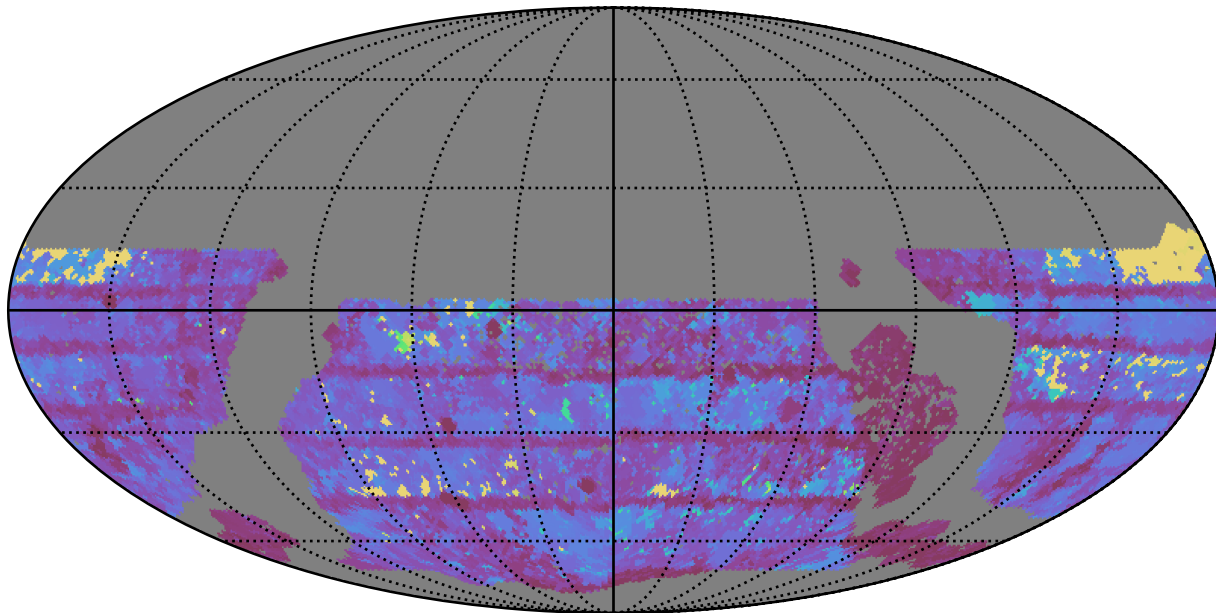
too_elab_r64_d2_giz_v3.4_10yrs WFD r band: Max Inter-Night Gap
