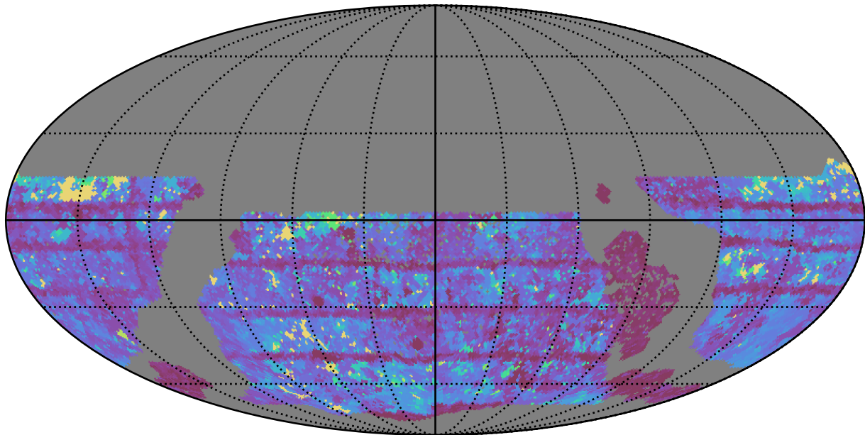
too_elab_r64_d2_giz_v3.4_10yrs WFD i band: Max Inter-Night Gap
