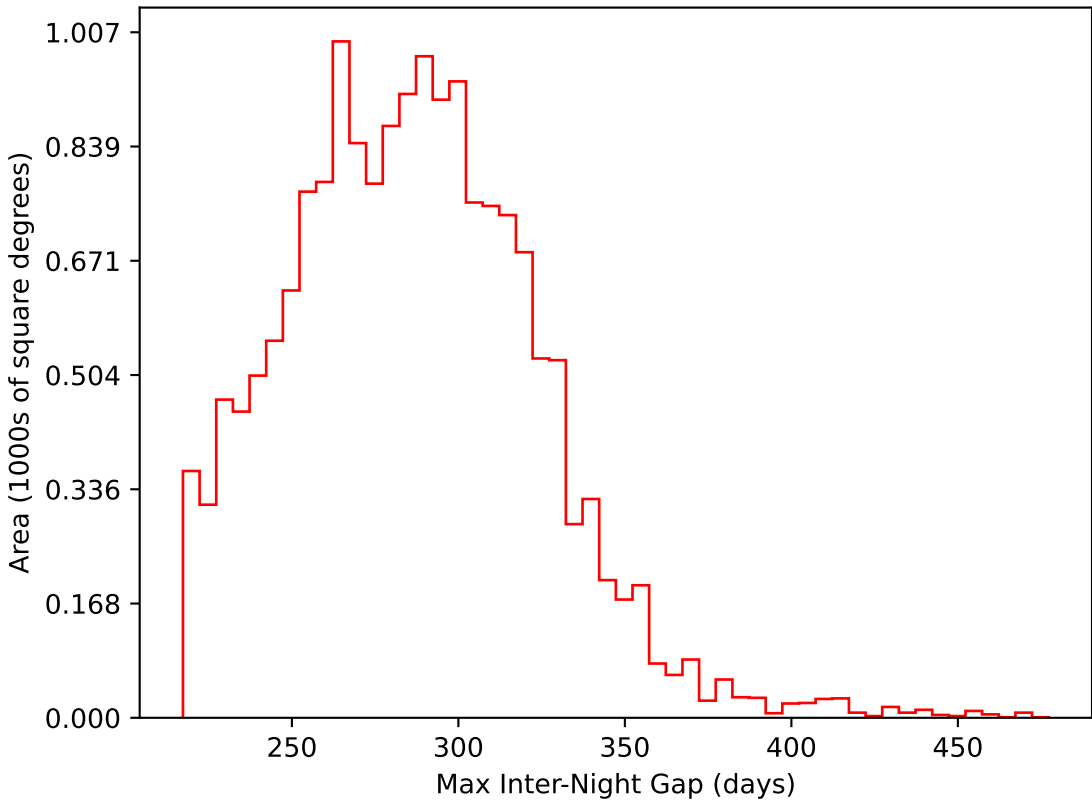
too_elab_r64_d2_giz_v3.4_10yrs WFD i band: Max Inter-Night Gap
