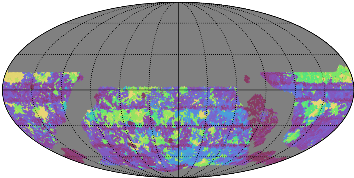
too_elab_r64_d2_giz_v3.4_10yrs WFD g band: Max Inter-Night Gap
