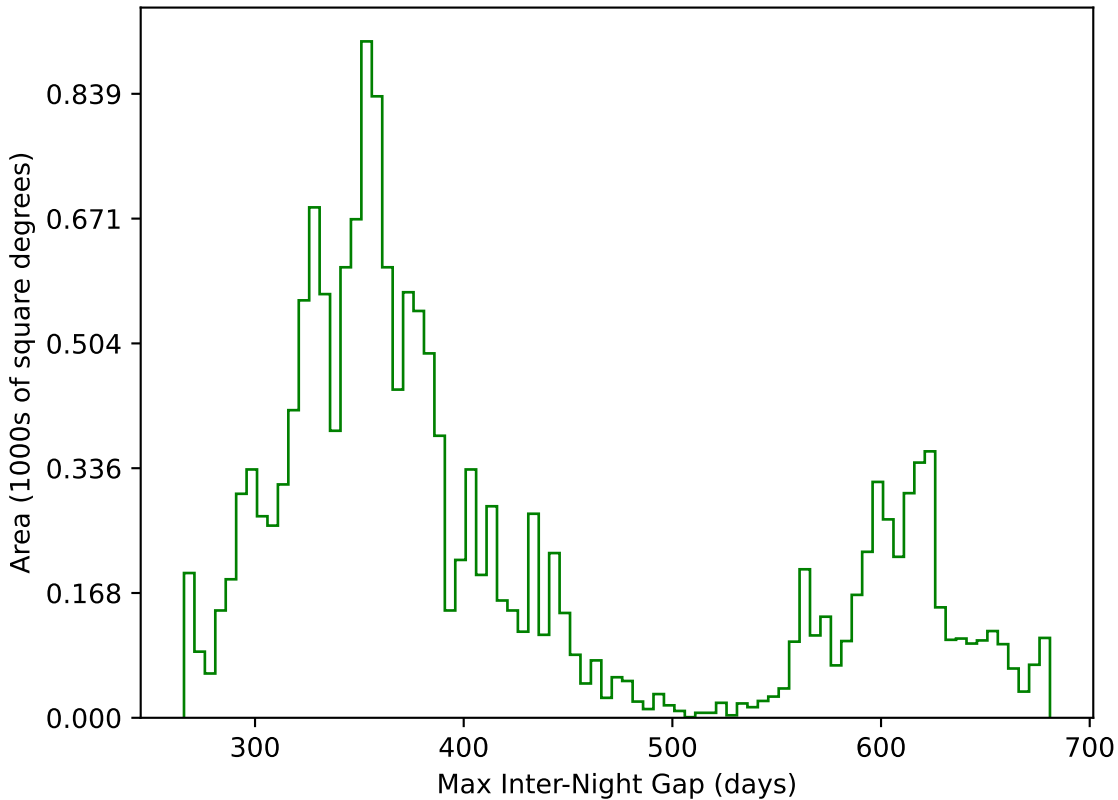
too_elab_r64_d2_giz_v3.4_10yrs WFD g band: Max Inter-Night Gap
