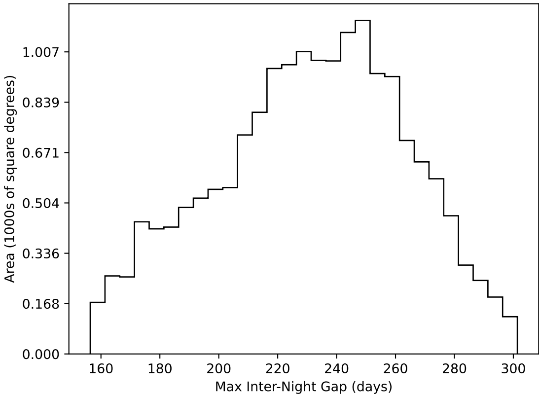
too_elab_r64_d2_giz_v3.4_10yrs WFD all bands: Max Inter-Night Gap
