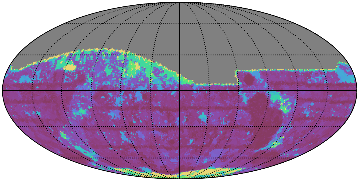
too_elab_r64_d2_giz_v3.4_10yrs All sky z band: Max Inter-Night Gap
