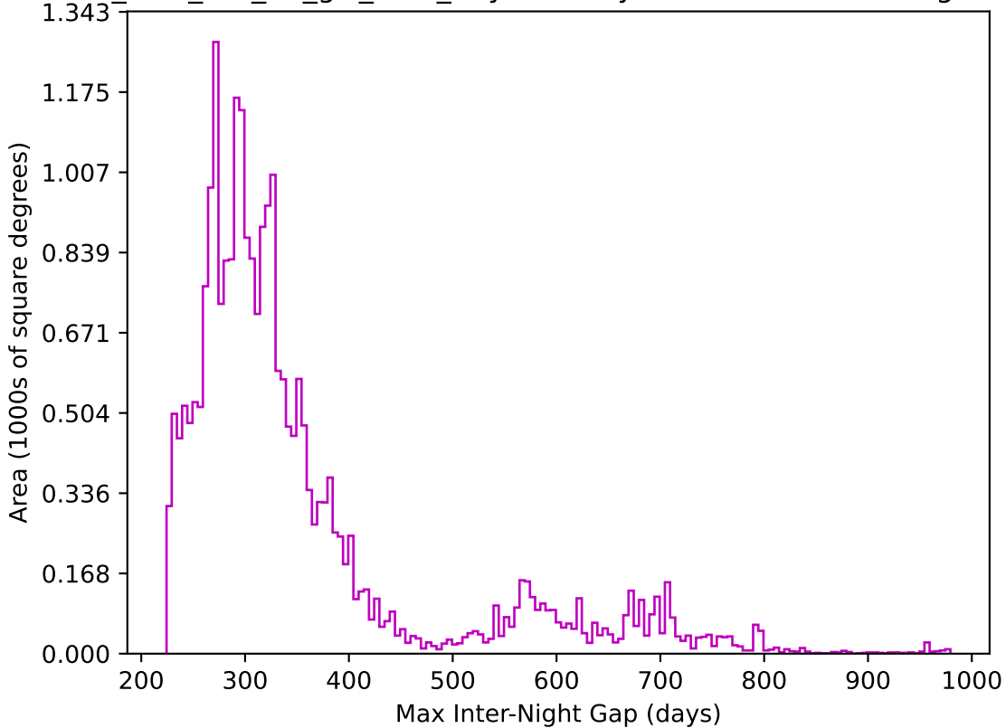
too_elab_r64_d2_giz_v3.4_10yrs All sky z band: Max Inter-Night Gap
