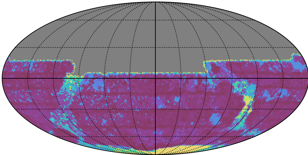
too_elab_r64_d2_giz_v3.4_10yrs All sky y band: Max Inter-Night Gap
