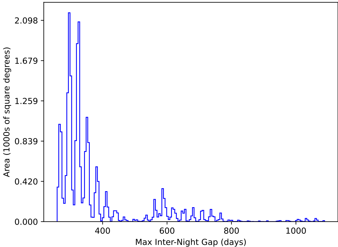
too_elab_r64_d2_giz_v3.4_10yrs All sky y band: Max Inter-Night Gap
