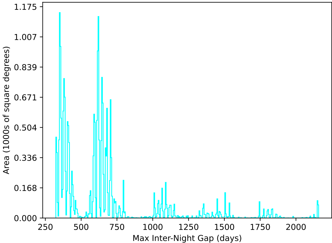
too_elab_r64_d2_giz_v3.4_10yrs All sky u band: Max Inter-Night Gap
