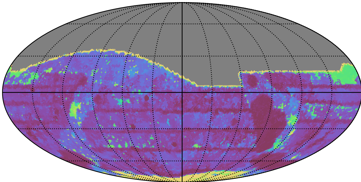
too_elab_r64_d2_giz_v3.4_10yrs All sky r band: Max Inter-Night Gap
