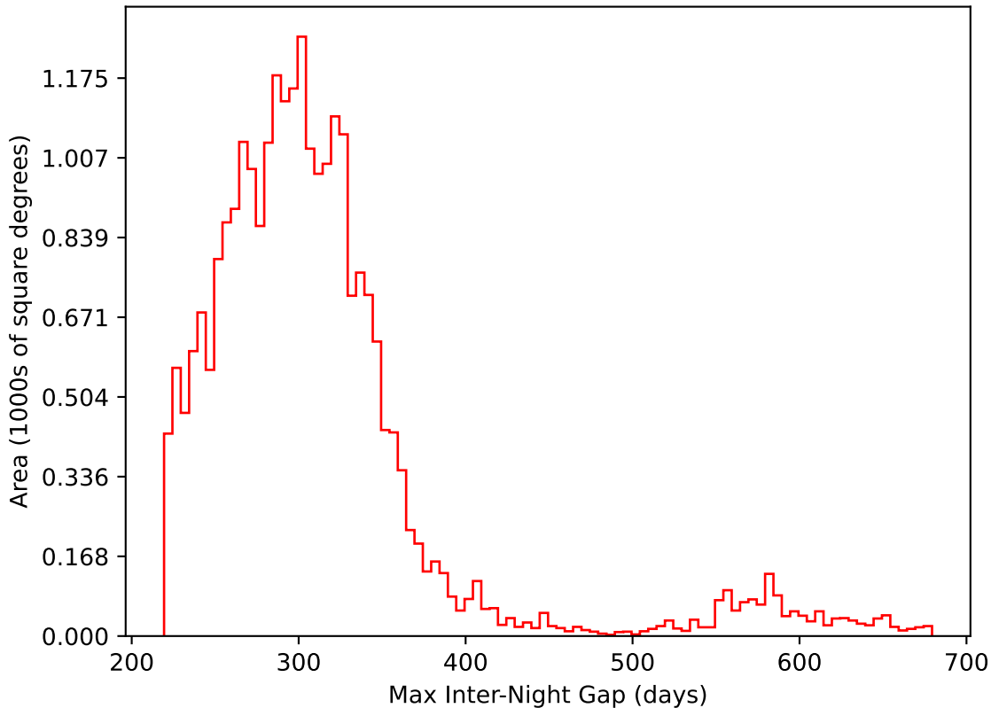
too_elab_r64_d2_giz_v3.4_10yrs All sky i band: Max Inter-Night Gap
