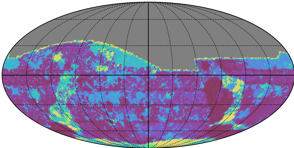
too_elab_r64_d2_giz_v3.4_10yrs All sky g band: Max Inter-Night Gap
