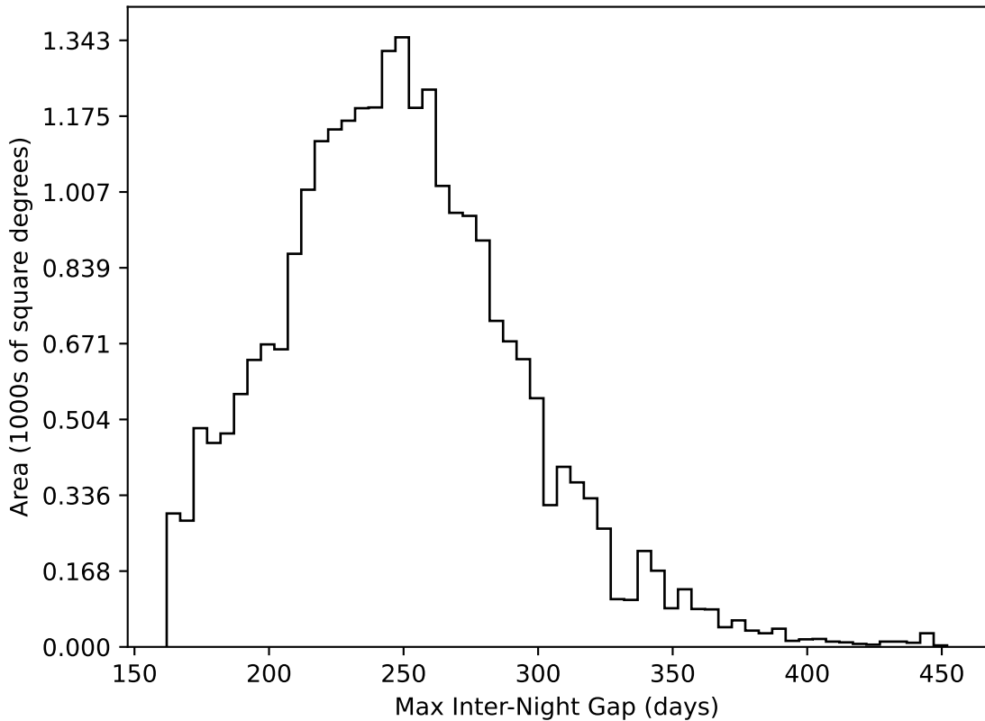
too_elab_r64_d2_giz_v3.4_10yrs All sky all bands: Max Inter-Night Gap
