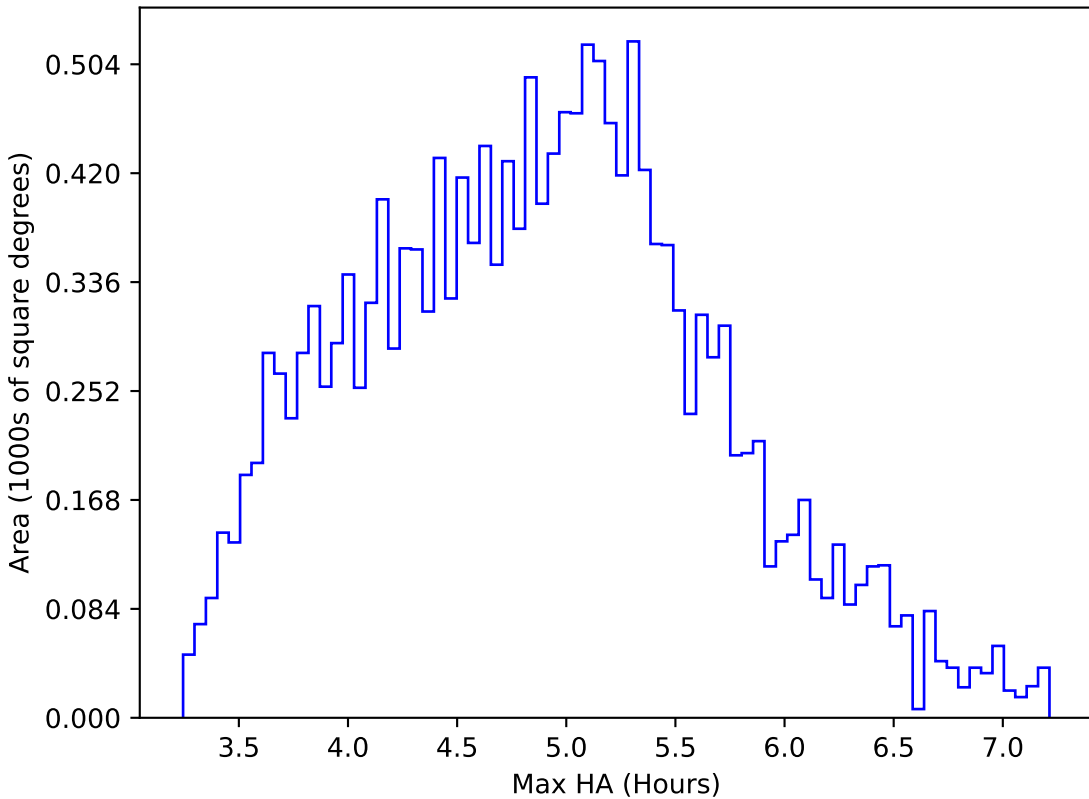
too_elab_r64_d2_giz_v3.4_10yrs WFD z band: Max HA
