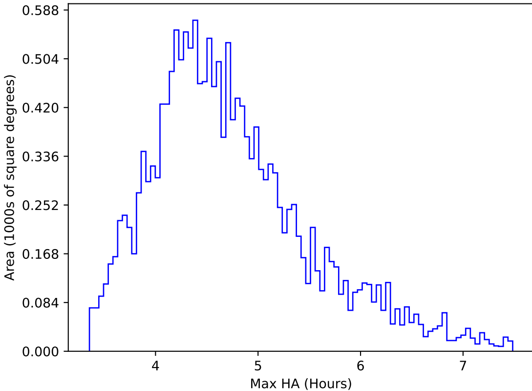
too_elab_r64_d2_giz_v3.4_10yrs WFD y band: Max HA
