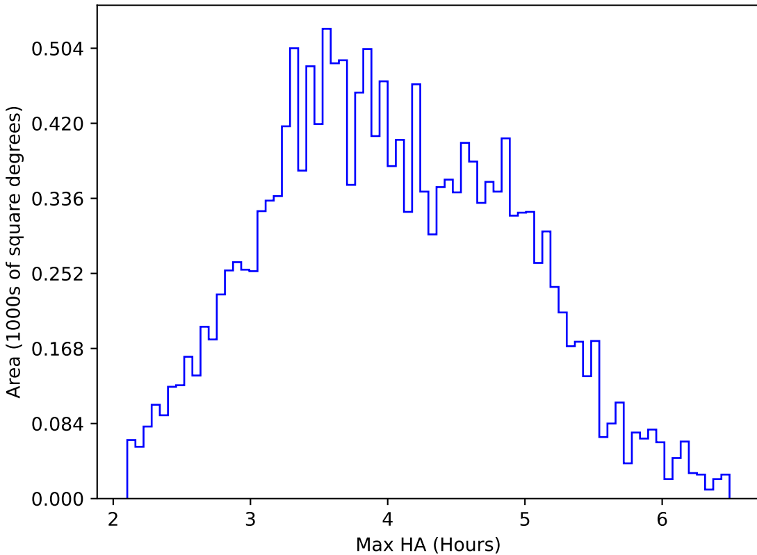
too_elab_r64_d2_giz_v3.4_10yrs WFD u band: Max HA
