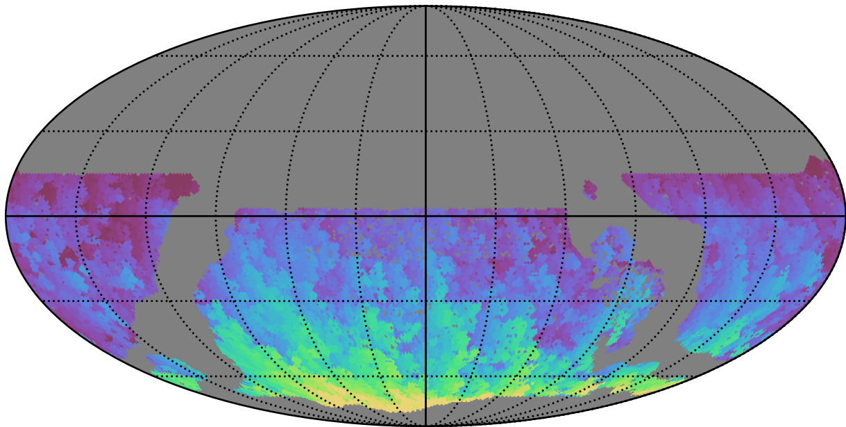
too_elab_r64_d2_giz_v3.4_10yrs WFD r band: Max HA
