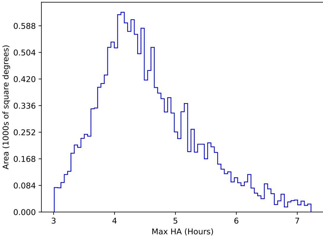
too_elab_r64_d2_giz_v3.4_10yrs WFD r band: Max HA
