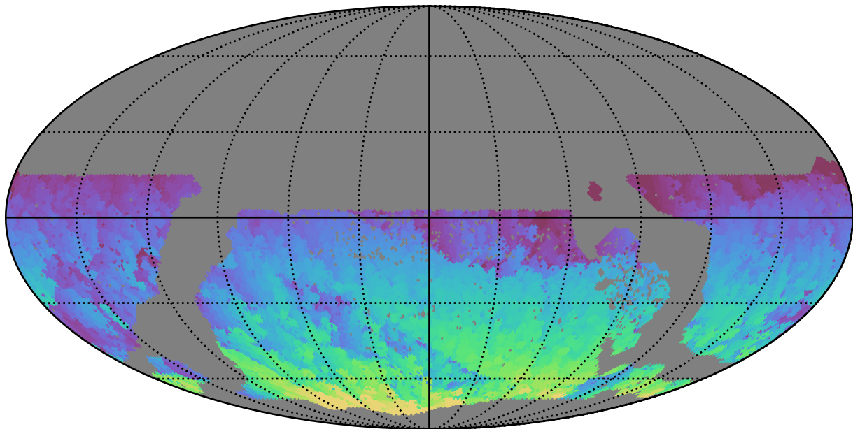
too_elab_r64_d2_giz_v3.4_10yrs WFD i band: Max HA
