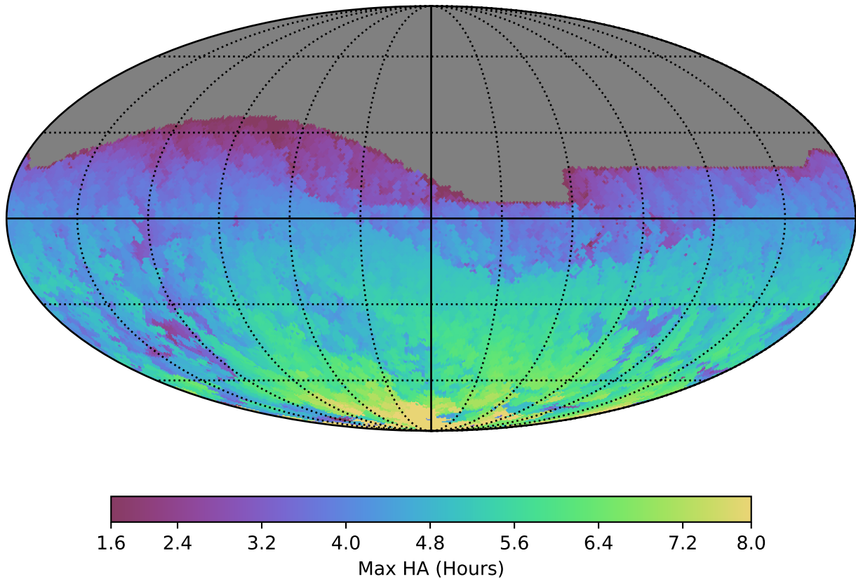
too_elab_r64_d2_giz_v3.4_10yrs All sky z band: Max HA
