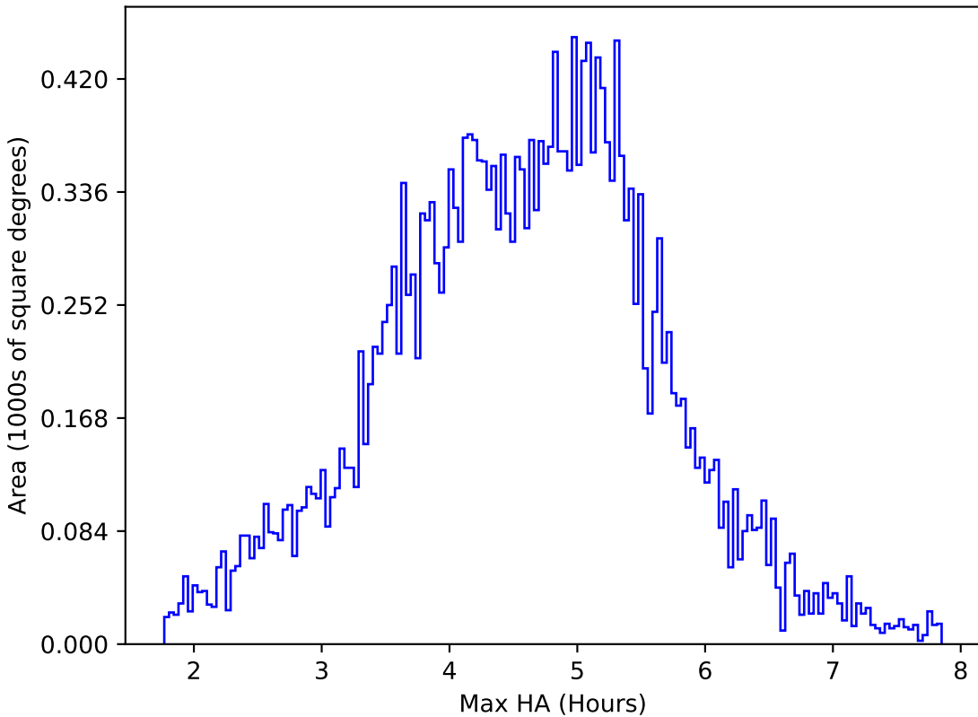
too_elab_r64_d2_giz_v3.4_10yrs All sky z band: Max HA
