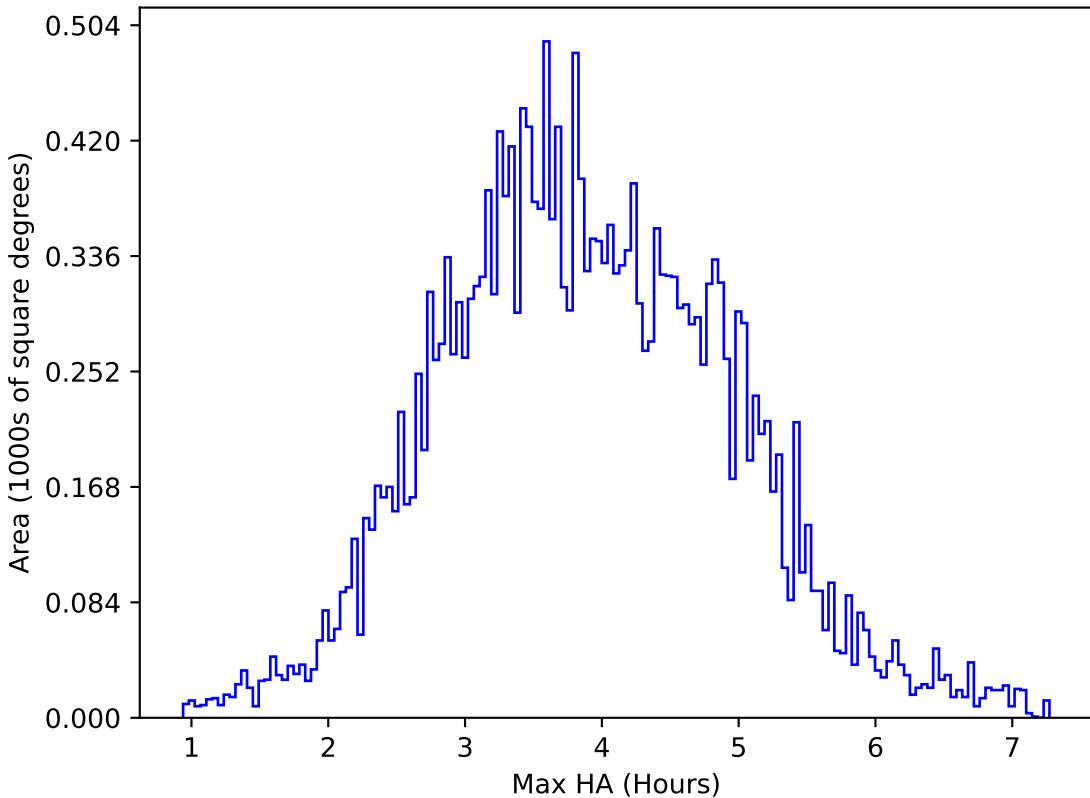
too_elab_r64_d2_giz_v3.4_10yrs All sky u band: Max HA
