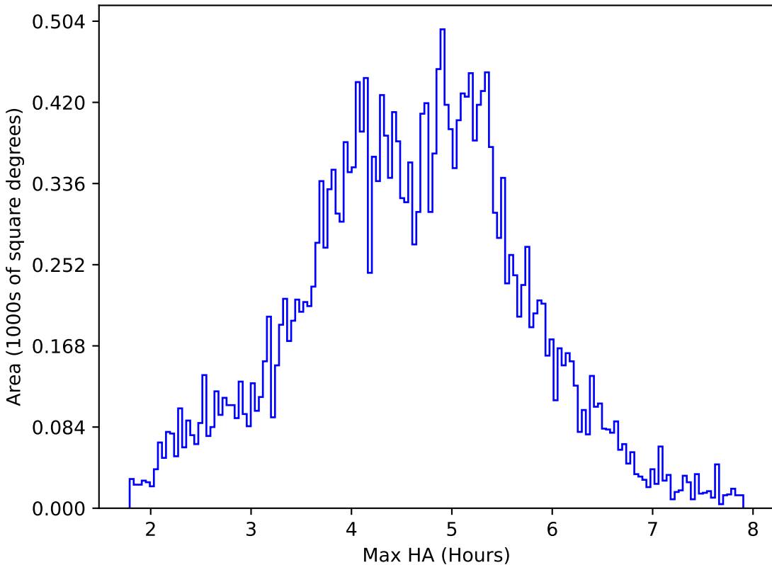
too_elab_r64_d2_giz_v3.4_10yrs All sky i band: Max HA
