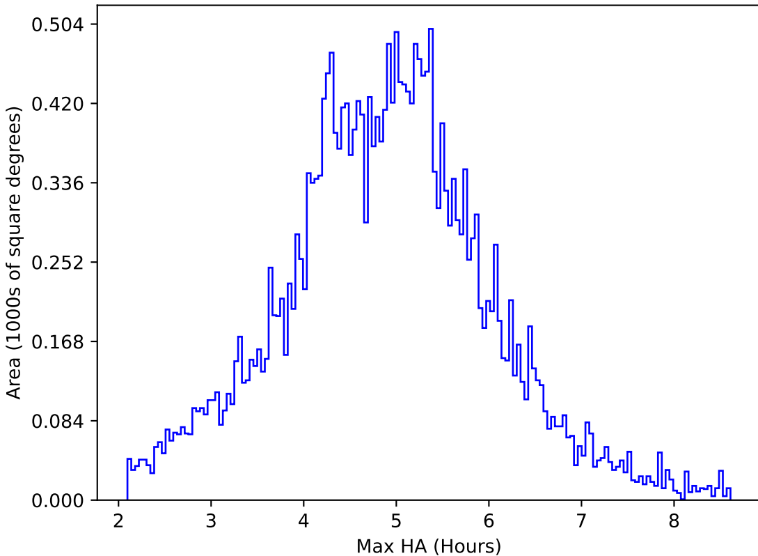
too_elab_r64_d2_giz_v3.4_10yrs All sky all bands: Max HA
