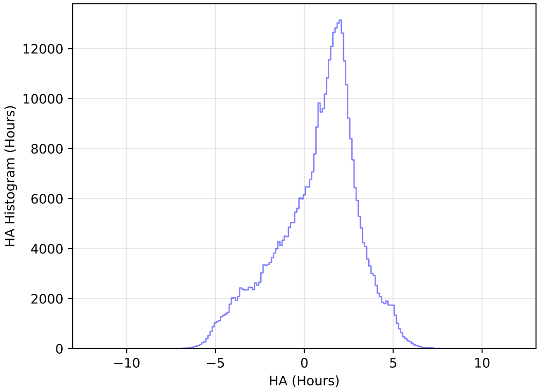
too_elab_r64_d2_giz_v3.4_10yrs WFD z band: HA Histogram
