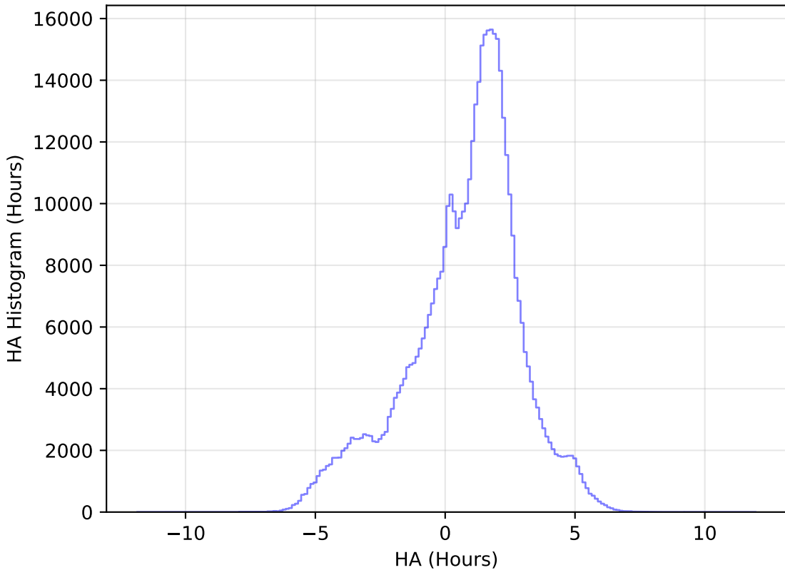
too_elab_r64_d2_giz_v3.4_10yrs WFD i band: HA Histogram
