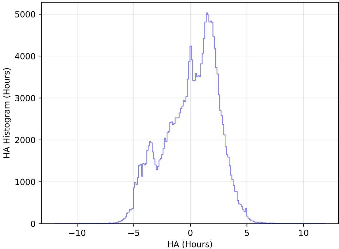
too_elab_r64_d2_giz_v3.4_10yrs WFD g band: HA Histogram
