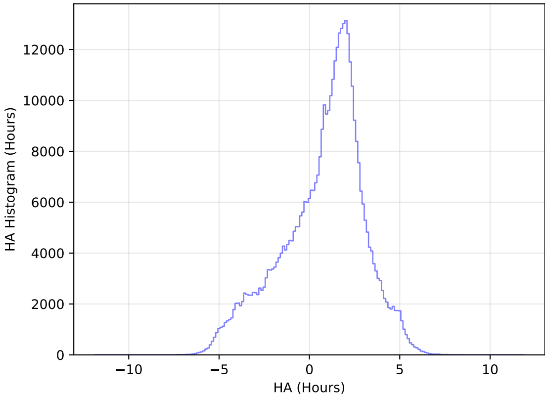
too_elab_r64_d2_giz_v3.4_10yrs All sky z band: HA Histogram
