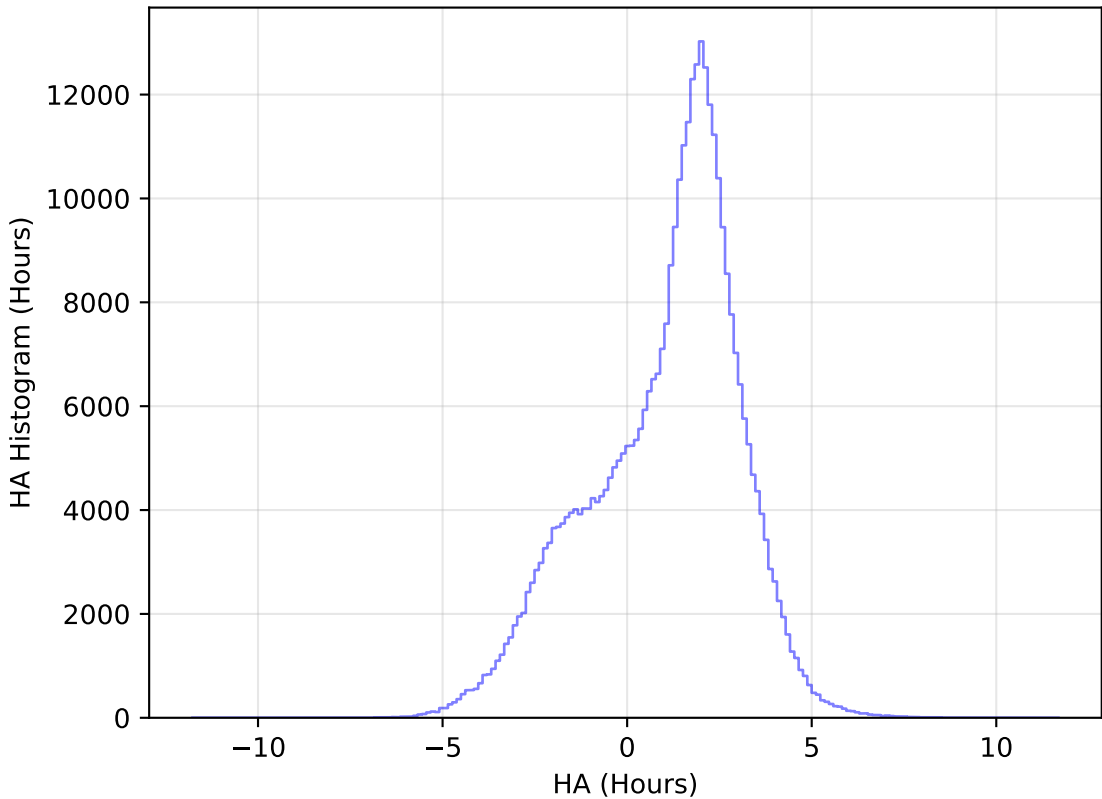
too_elab_r64_d2_giz_v3.4_10yrs All sky y band: HA Histogram
