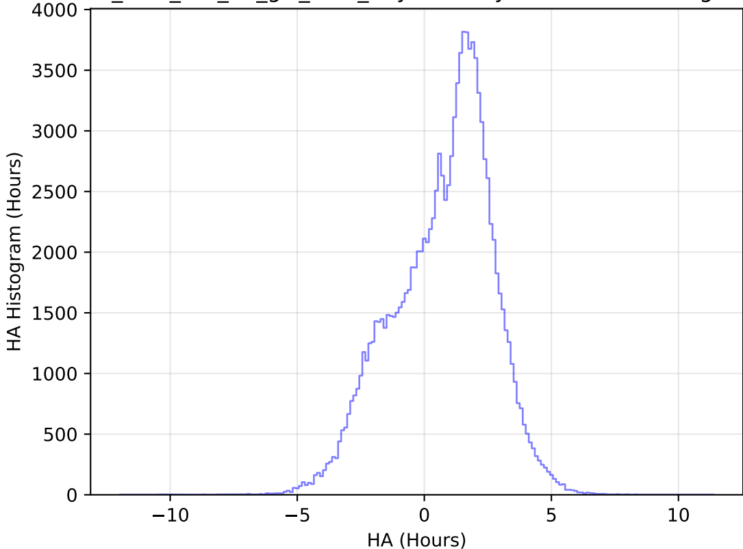
too_elab_r64_d2_giz_v3.4_10yrs All sky u band: HA Histogram
