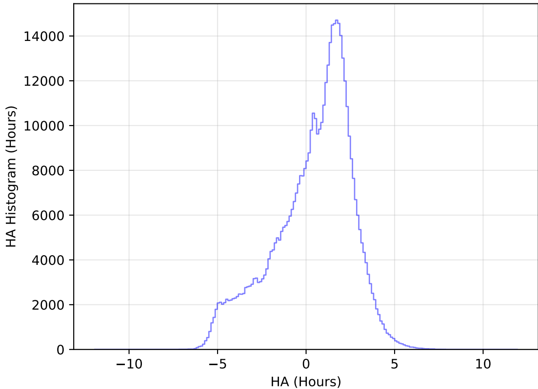
too_elab_r64_d2_giz_v3.4_10yrs All sky r band: HA Histogram
