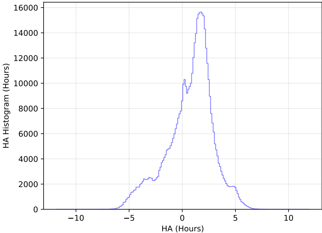
too_elab_r64_d2_giz_v3.4_10yrs All sky i band: HA Histogram
