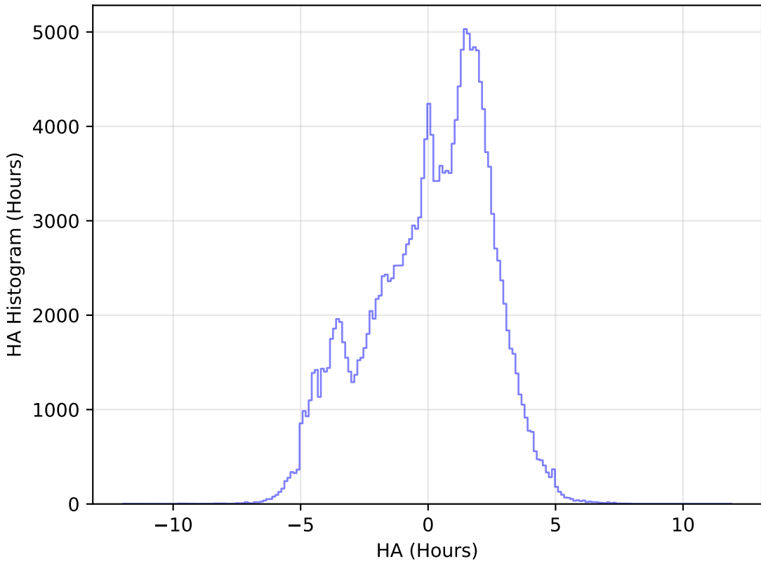
too_elab_r64_d2_giz_v3.4_10yrs All sky g band: HA Histogram
