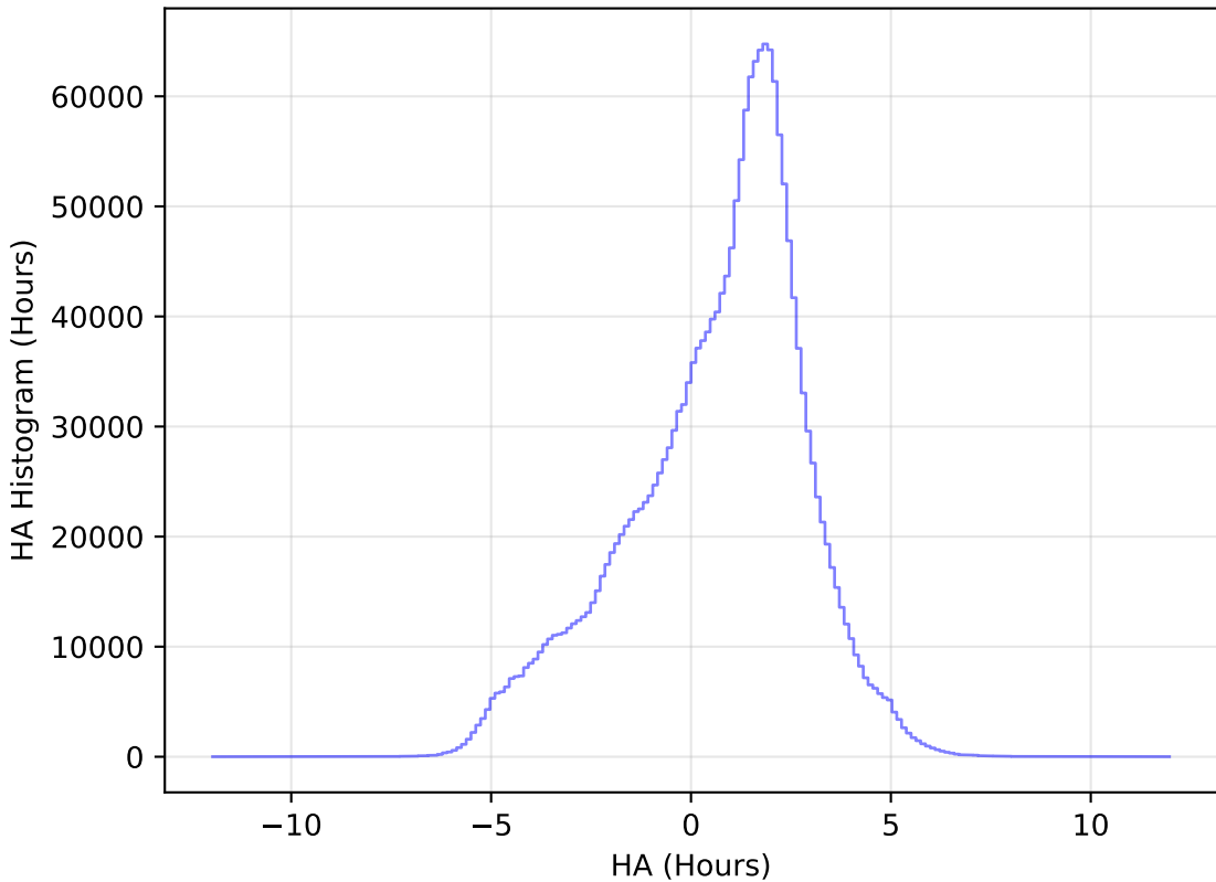
too_elab_r64_d2_giz_v3.4_10yrs All sky all bands: HA Histogram
