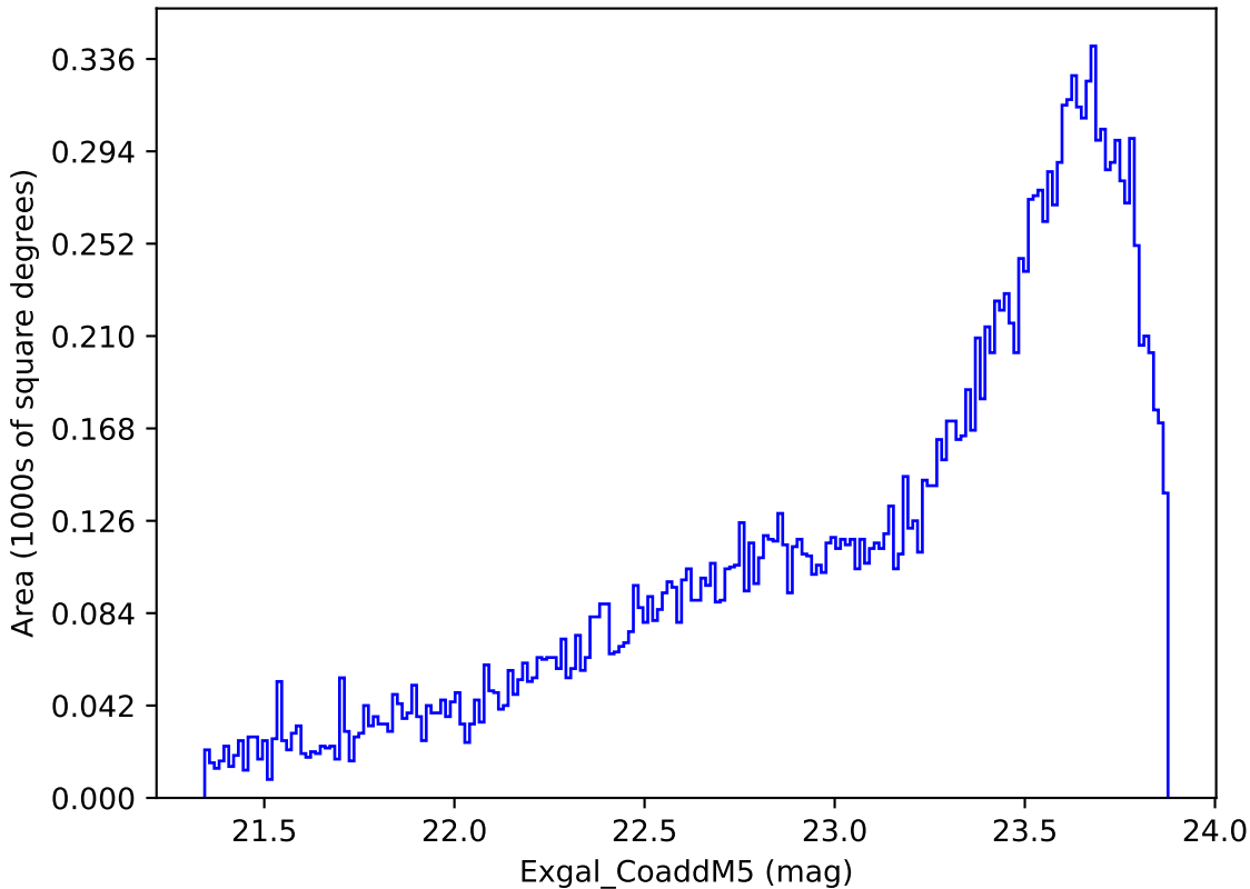
too_elab_r64_d2_giz_v3.4_10yrs Yr 3-4 y band: Exgal_CoaddM5
