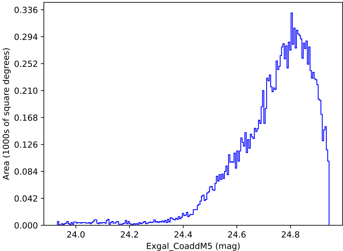
too_elab_r64_d2_giz_v3.4_10yrs WFD y band: Exgal_CoaddM5
