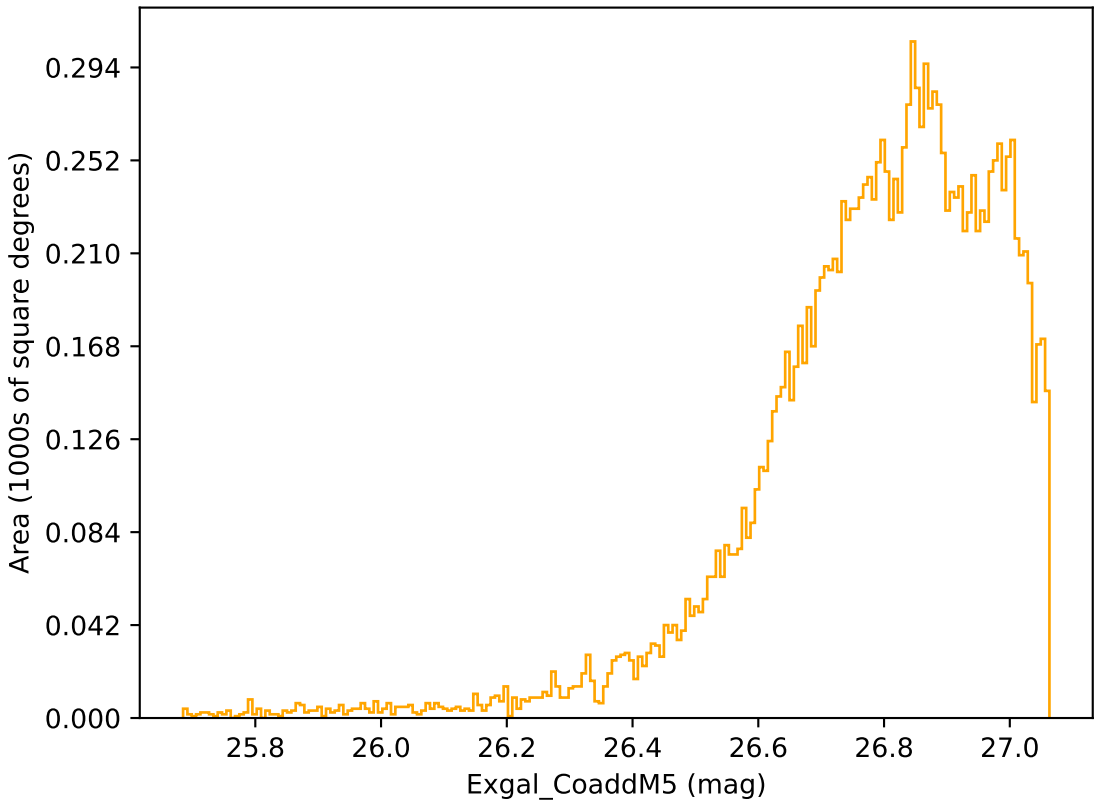
too_elab_r64_d2_giz_v3.4_10yrs WFD r band: Exgal_CoaddM5
