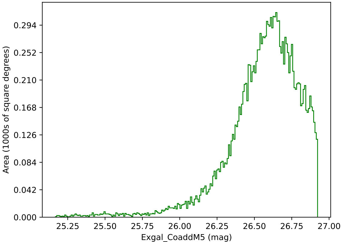
too_elab_r64_d2_giz_v3.4_10yrs WFD g band: Exgal_CoaddM5
