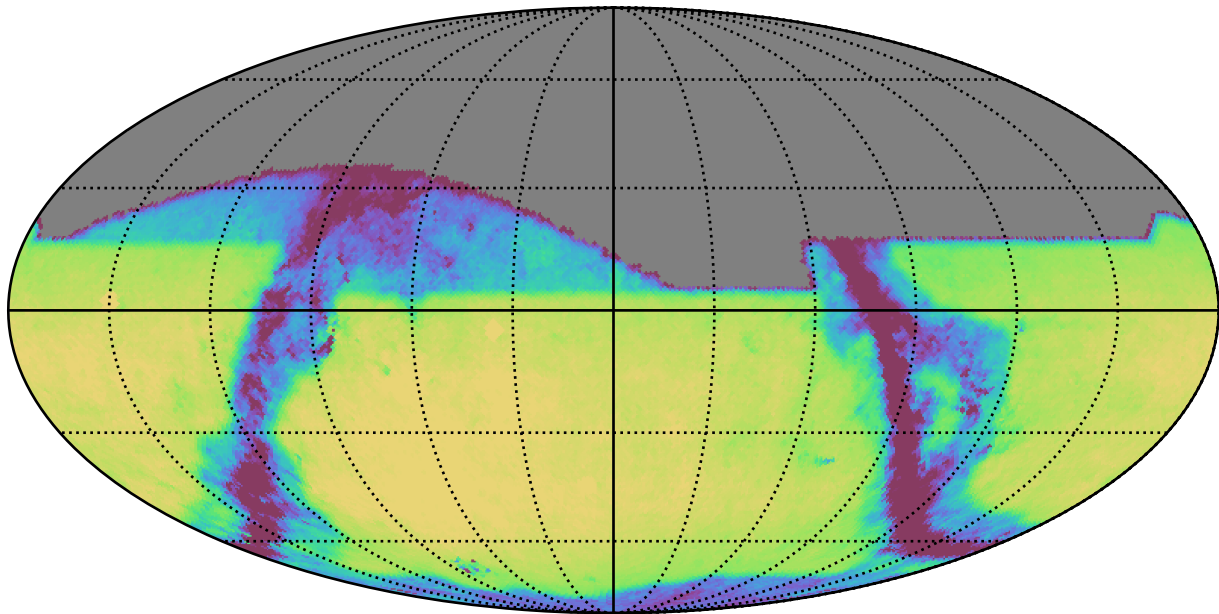
too_elab_r64_d2_giz_v3.4_10yrs All sky z band: Exgal_CoaddM5
