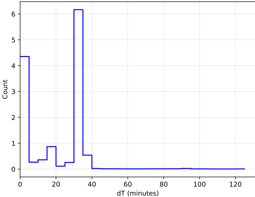
too_elab_r64_d2_giz_v3.4_10yrs All sky: DeltaT Histogram 1e6
