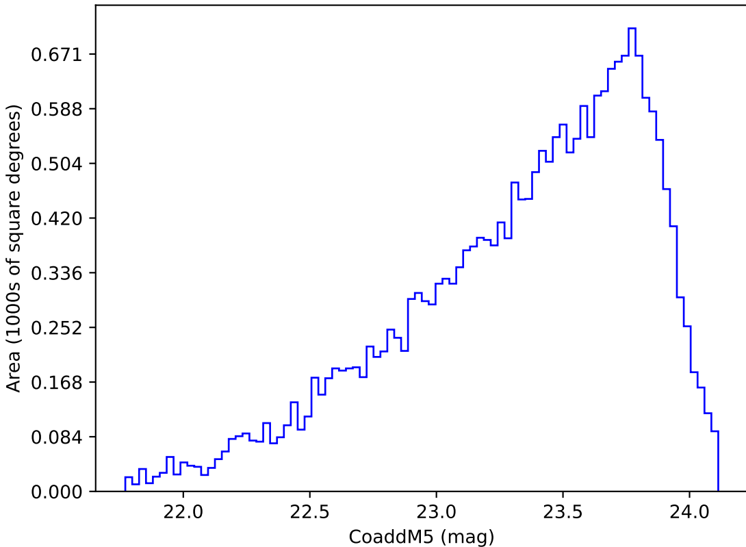
too_elab_r64_d2_giz_v3.4_10yrs Yr 3-4 y band: CoaddM5
