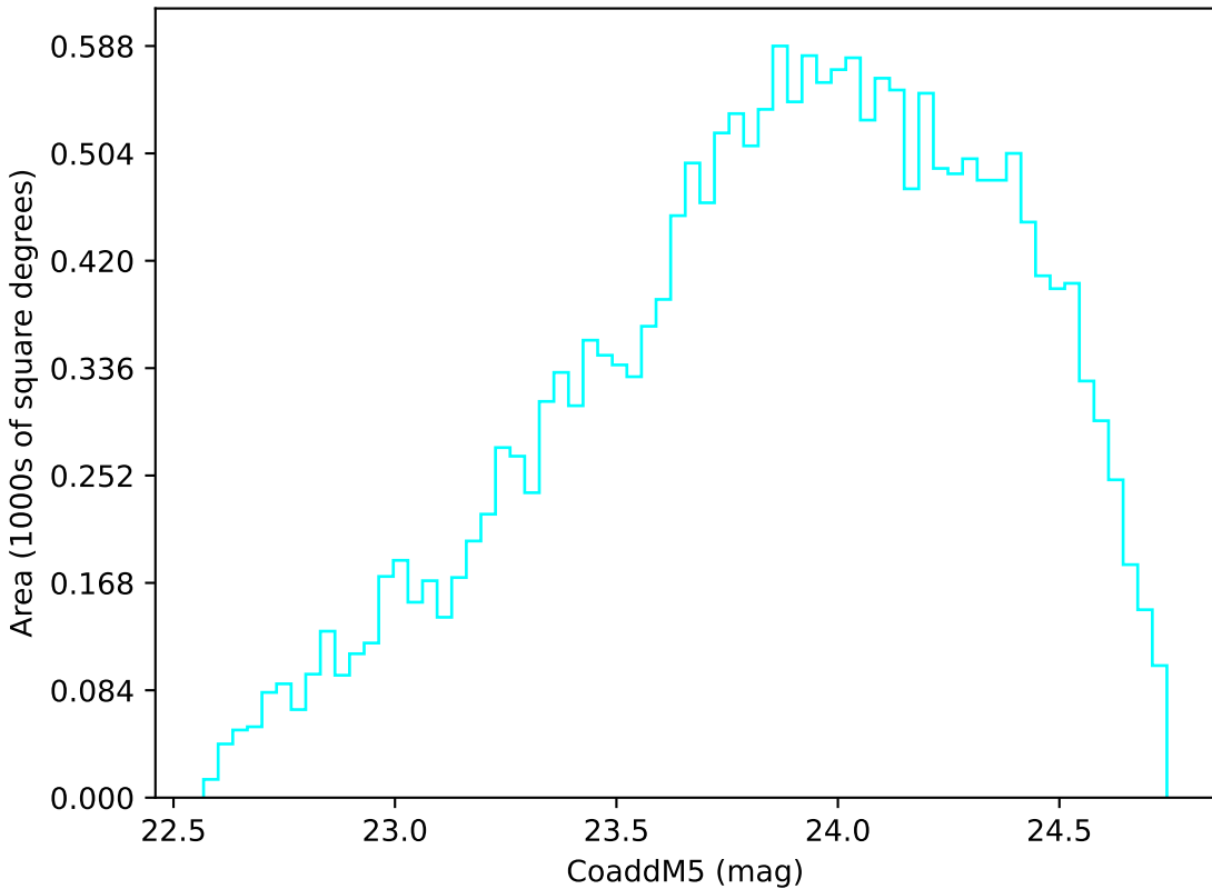
too_elab_r64_d2_giz_v3.4_10yrs Yr 3-4 u band: CoaddM5
