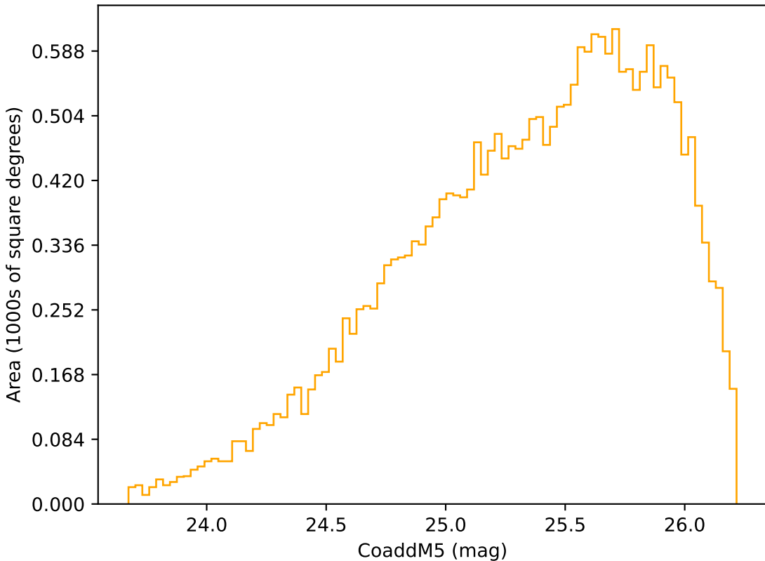
too_elab_r64_d2_giz_v3.4_10yrs Yr 3-4 r band: CoaddM5
