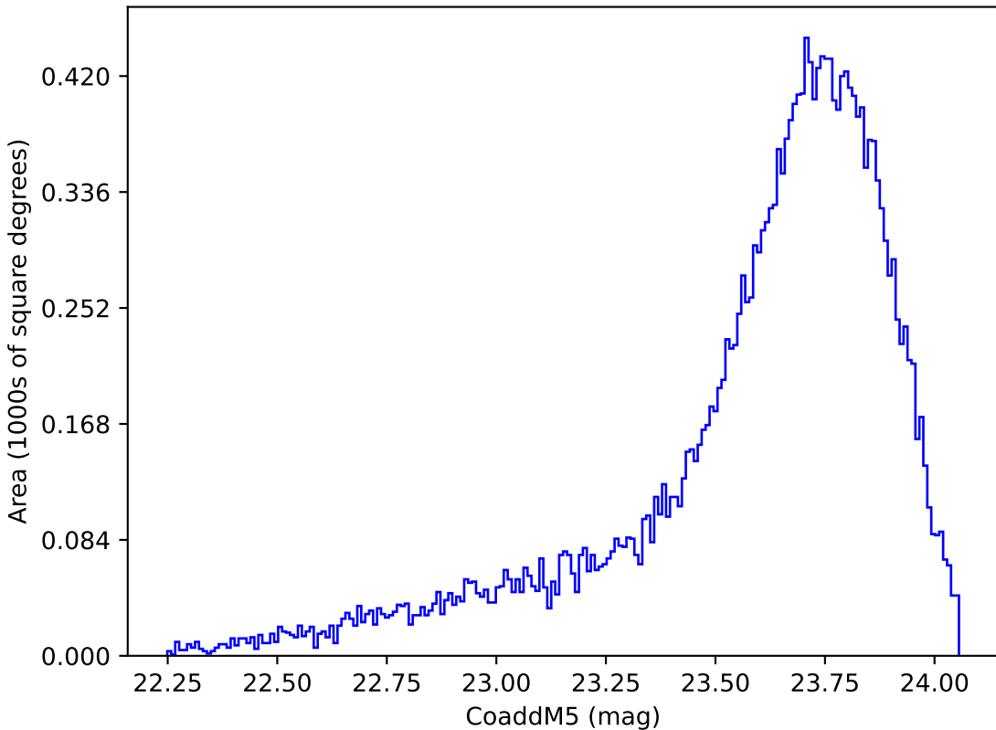
too_elab_r64_d2_giz_v3.4_10yrs Yr 1 y band: CoaddM5
