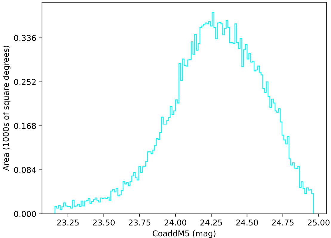
too_elab_r64_d2_giz_v3.4_10yrs Yr 1 u band: CoaddM5
