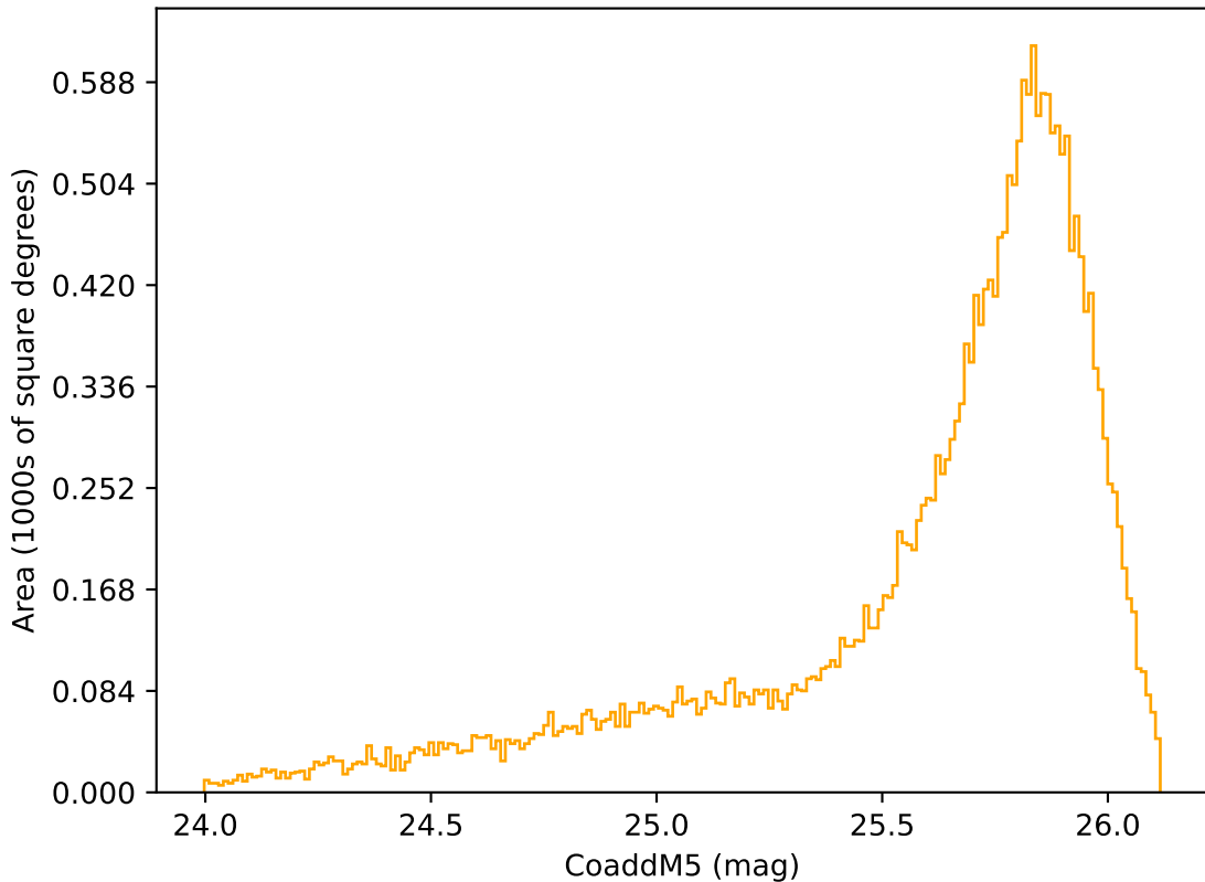
too_elab_r64_d2_giz_v3.4_10yrs Yr 1 r band: CoaddM5
