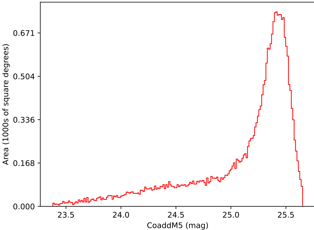
too_elab_r64_d2_giz_v3.4_10yrs Yr 1 i band: CoaddM5
